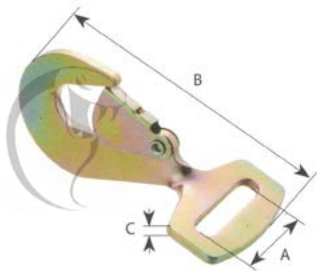
50MM/5T Twisted Snap Hook
